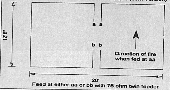
Fig. 7 G6XN Improvements to the VK2ABQ (20M Version)
